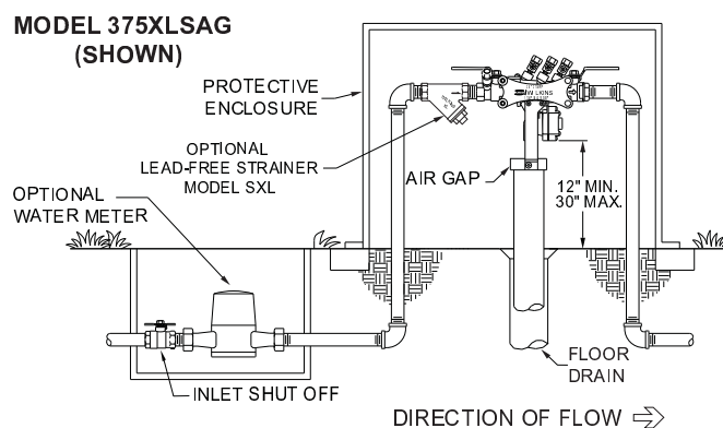
OUTDOOR INSTALLATION
