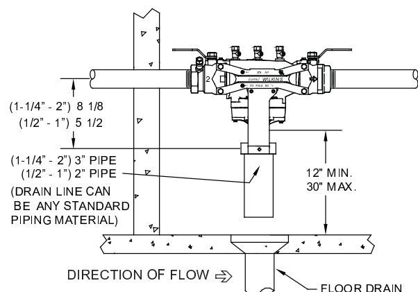
INDOOR INSTALLATION
